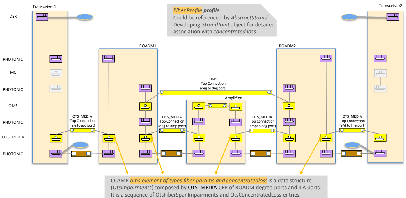
Figure 6-121 OTS Impairments
