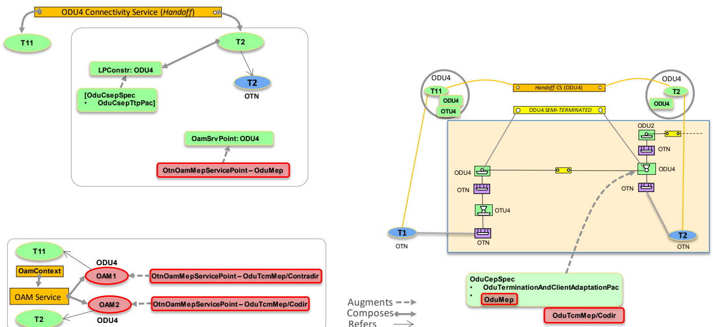
Figure 6-26 Asymmetric scenario 2: ODUk Handoff CS (OTN ENNI) - Part 2
