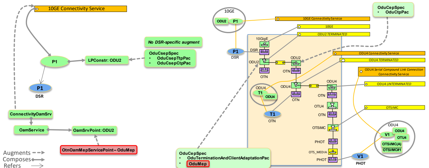
Figure 6-15 DSR/ODUj Connectivity Service on ODUk CS on ODUk SCLC CS
