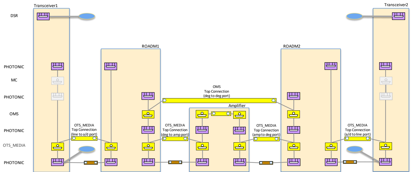
Figure 5-33 Scenario 2 : Integrated Management, time zero
