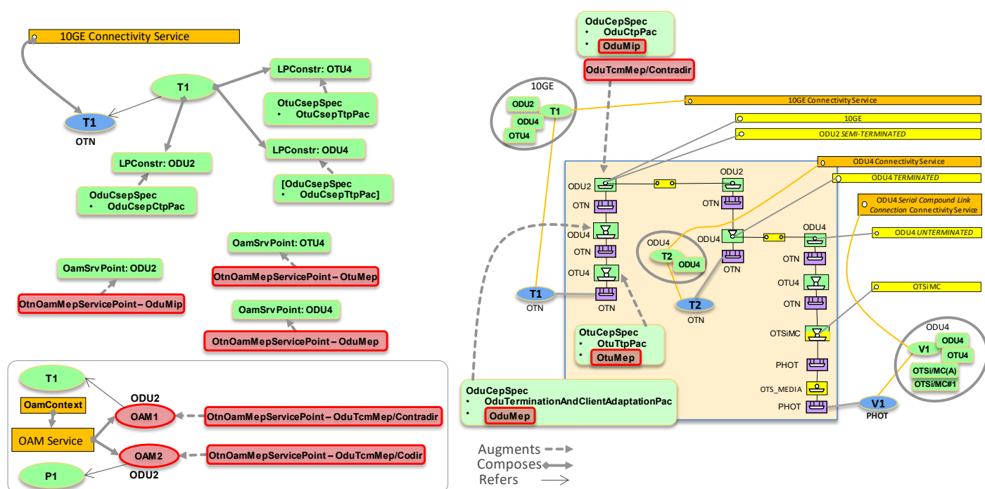
Figure 6-31 Asymmetric scenario 4: DSR/ODUj CS (OTN ENNI)
