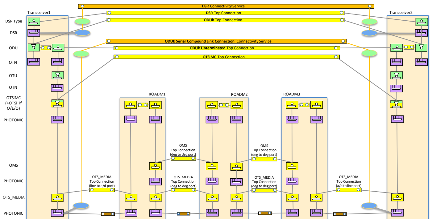
Figure 5-48 Scenario 2 : Integrated Management, OTSiMC+ODU CS, MC not represented
