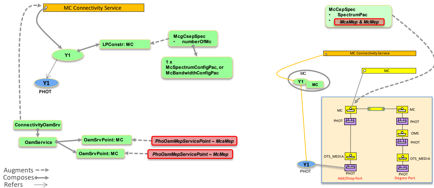
Figure 6-42 MC Connectivity Service at Add/Drop side
