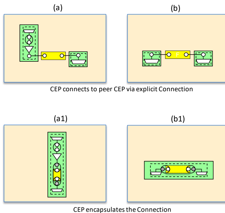
Figure 5-2 Explicit and encapsulated connections
