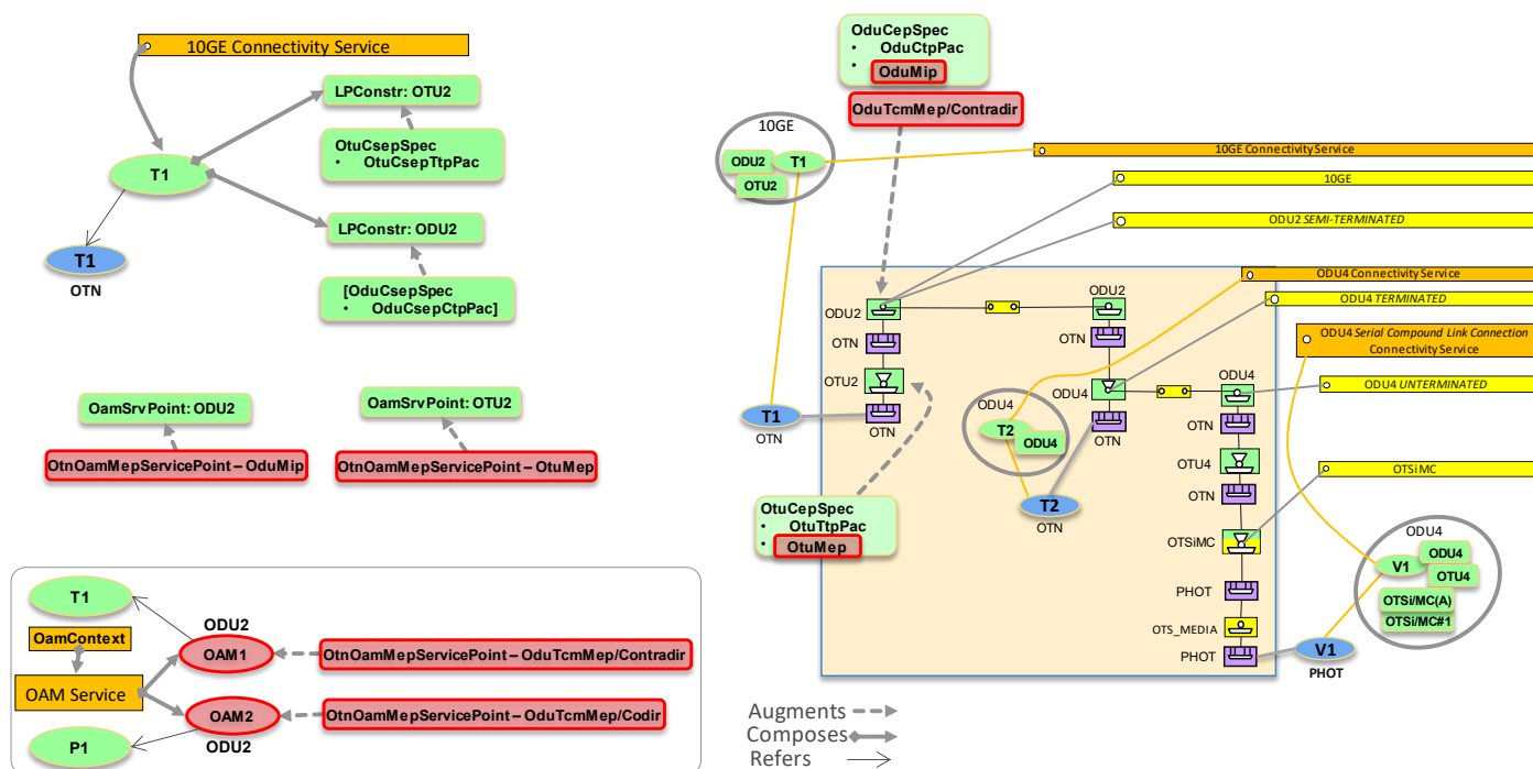
Figure 6-30 Asymmetric scenario 3: DSR/ODUj CS (OTN ENNI)
