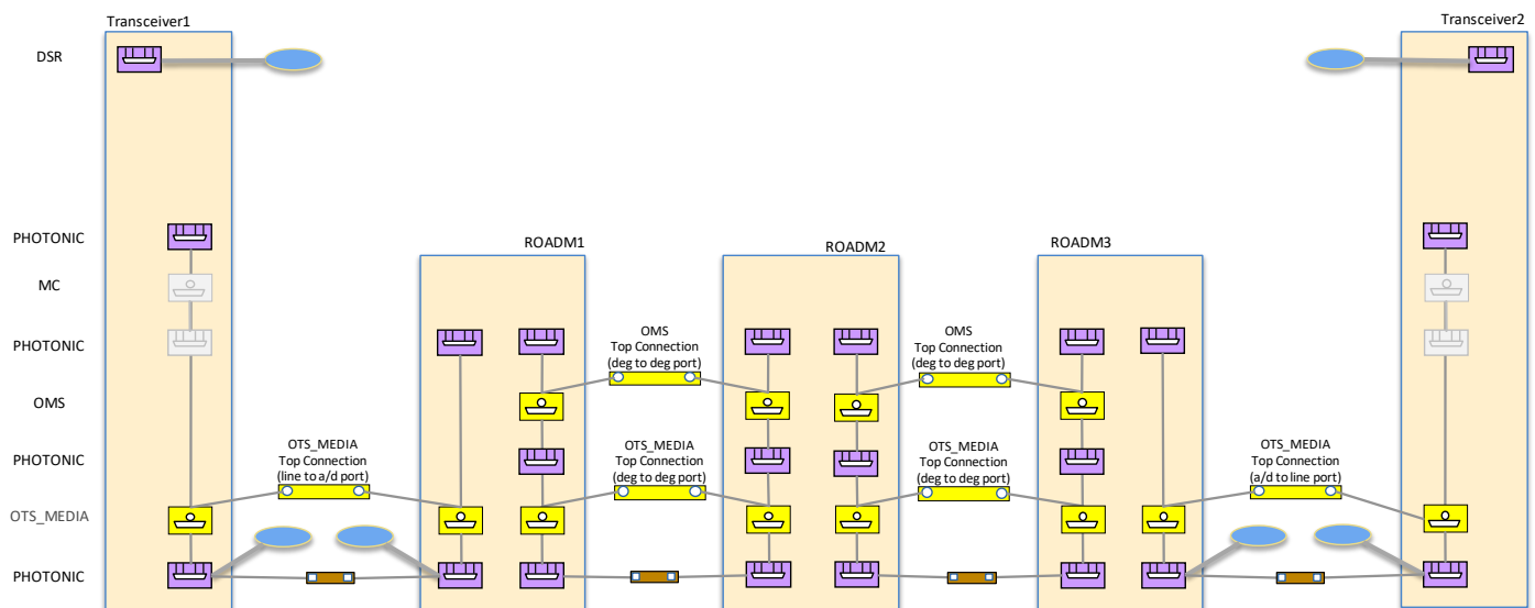
Figure 5-34 Scenario 2 : Integrated Management, time zero, SIPs at a/d ports
