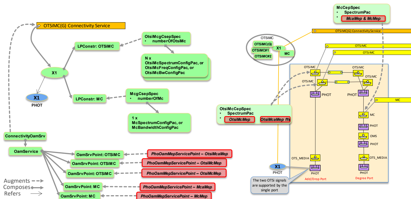
Figure 6-50 OTSiMCG CS, MC Connection automatically created at Degree side
