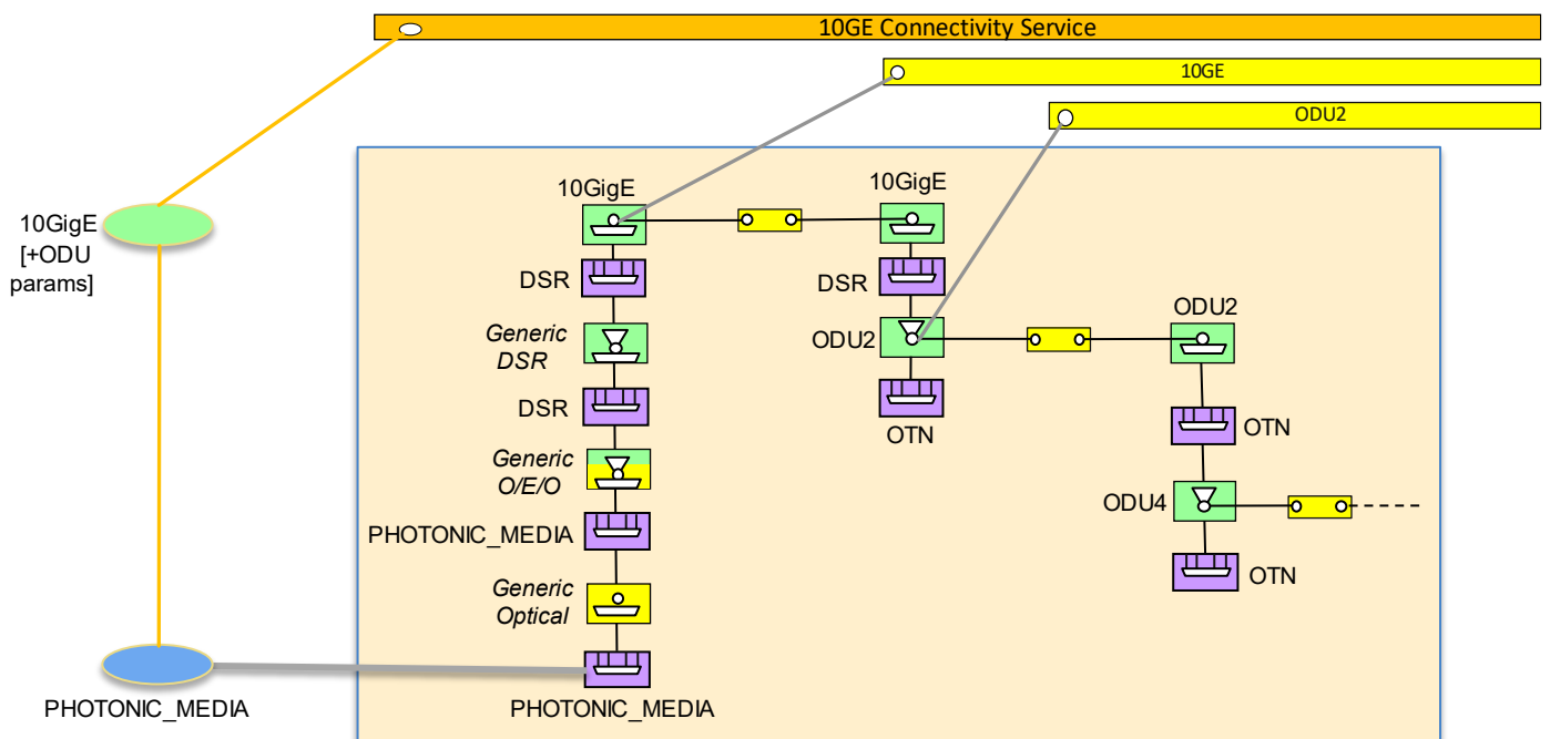
Figure 5-59 DSR UNI, explicit model of functions (optical)
