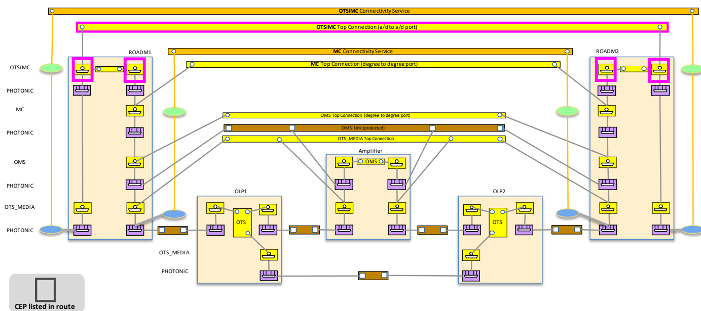
Figure 6-88 UC-5a OLP protection TAPI representation 1 – OTSiMC route
