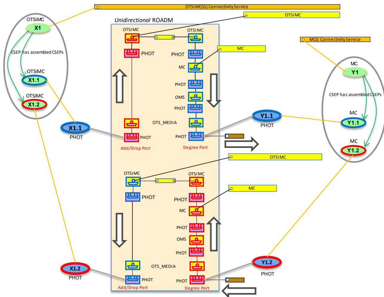
Figure 5-13 OTSiMC with unidirectional CSEPs, first case
