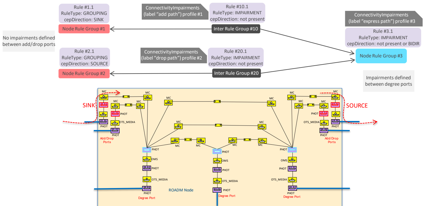
Figure 6-127 Conn. Impairments per add, drop and express conns, homogeneous between add / drop and express
