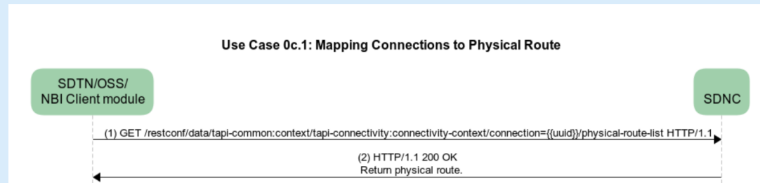
Figure 6-6: UC0c1 workflow
