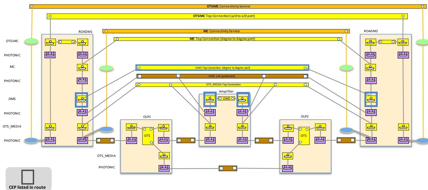
Figure 6-87 UC-5a OLP protection TAPI representation 1 – OMS route
