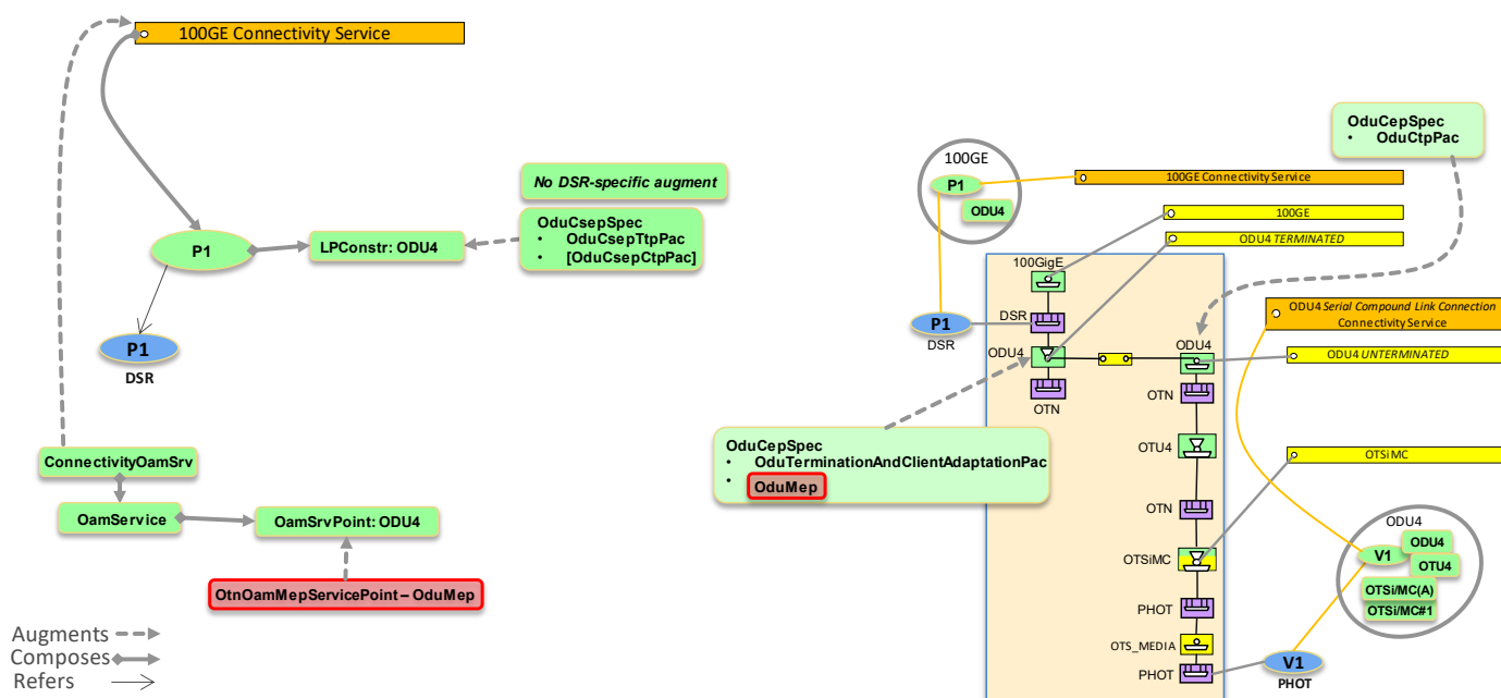
Figure 6-9 DSR/ODUk Connectivity Service on ODUk SCLC CS
