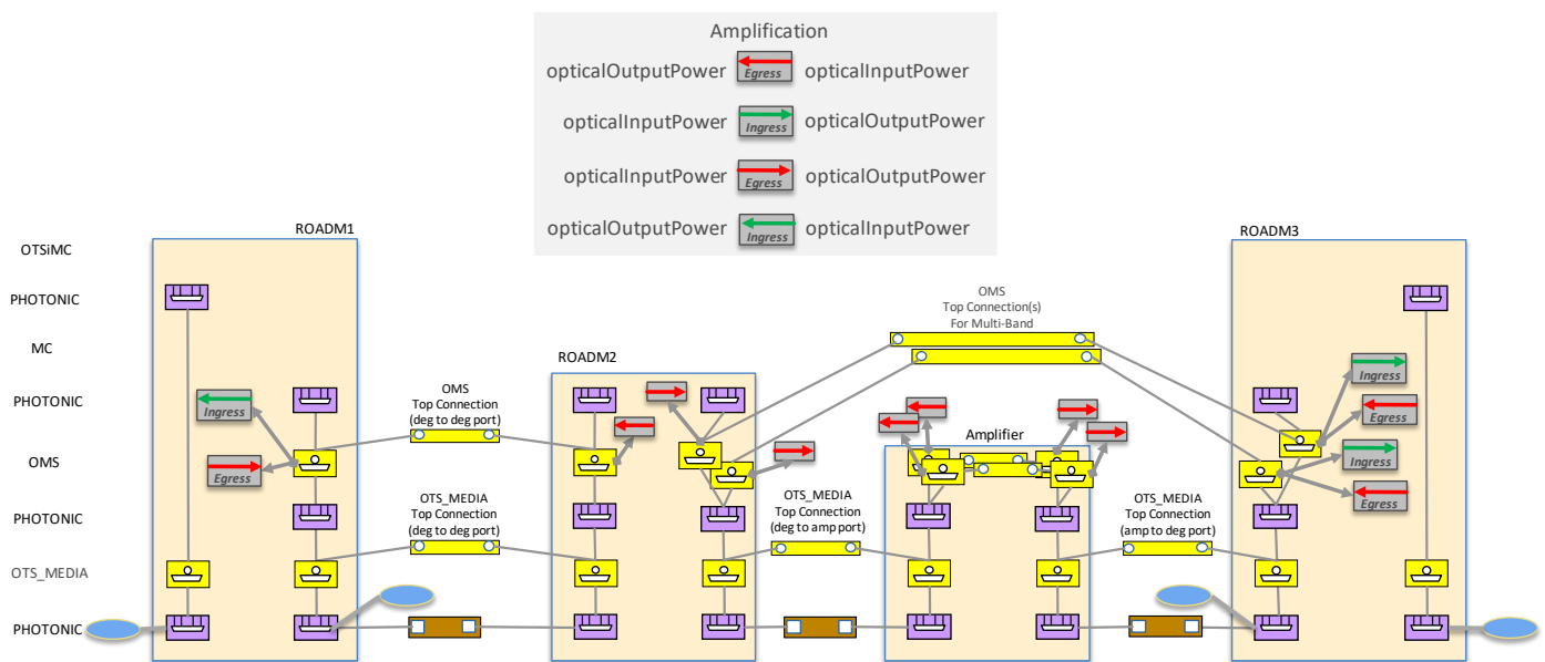
Figure 6-122 Amplification Impairments
