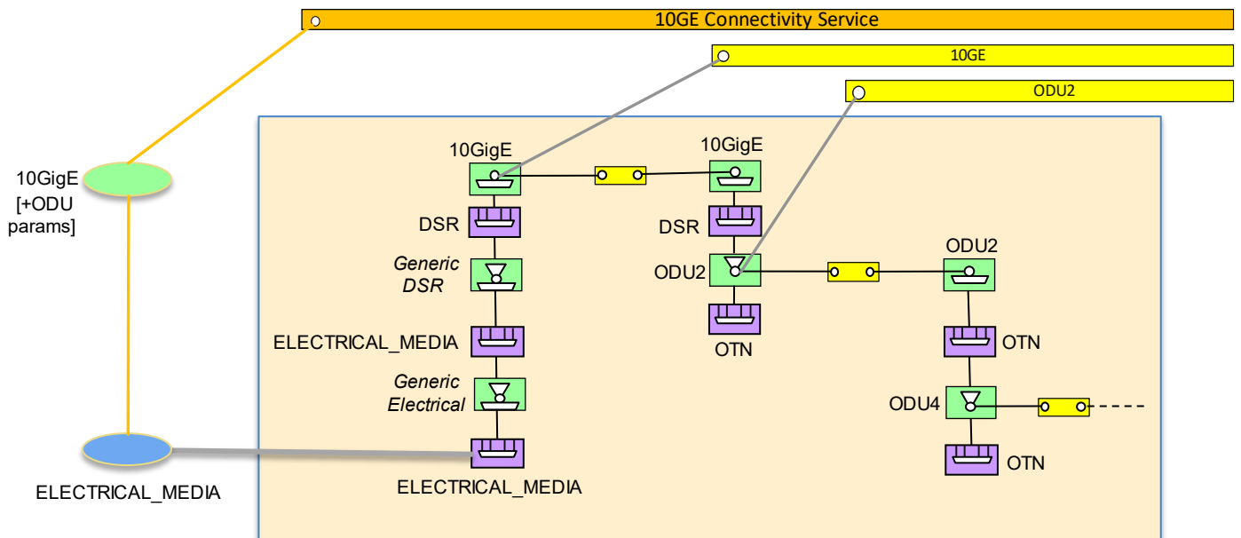
Figure 5-58 DSR UNI, explicit model of functions (electrical)
