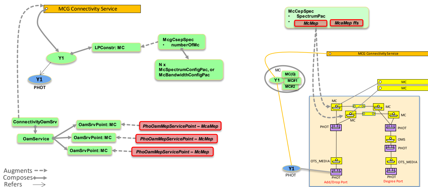
Figure 6-43 MCG Connectivity Service at Add/Drop side
